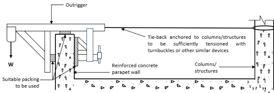
Fig 1b. Side section view showing outrigger, tie-back and anchorage point in line. Suspension and safety rope not shown.
